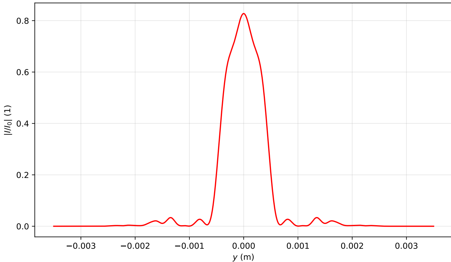
Intensity profile I(x=0, y, z=2.149)/I_0 , P_{in}=3.0P_{cr} , artificial time
